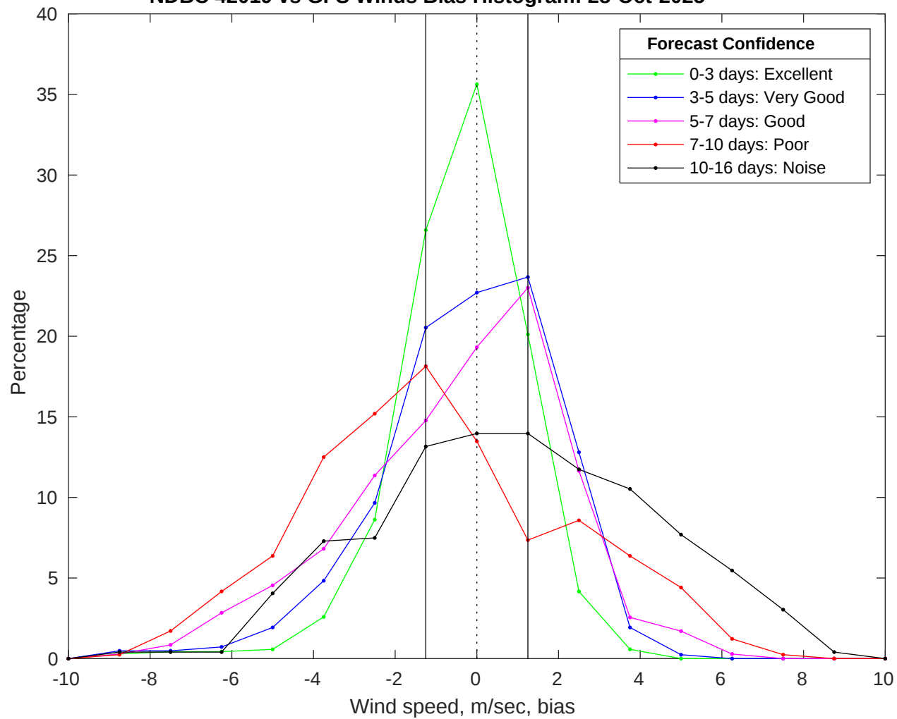
NDBC 42019 vs GFS Winds Bias Histogram: 28-Oct-2025
