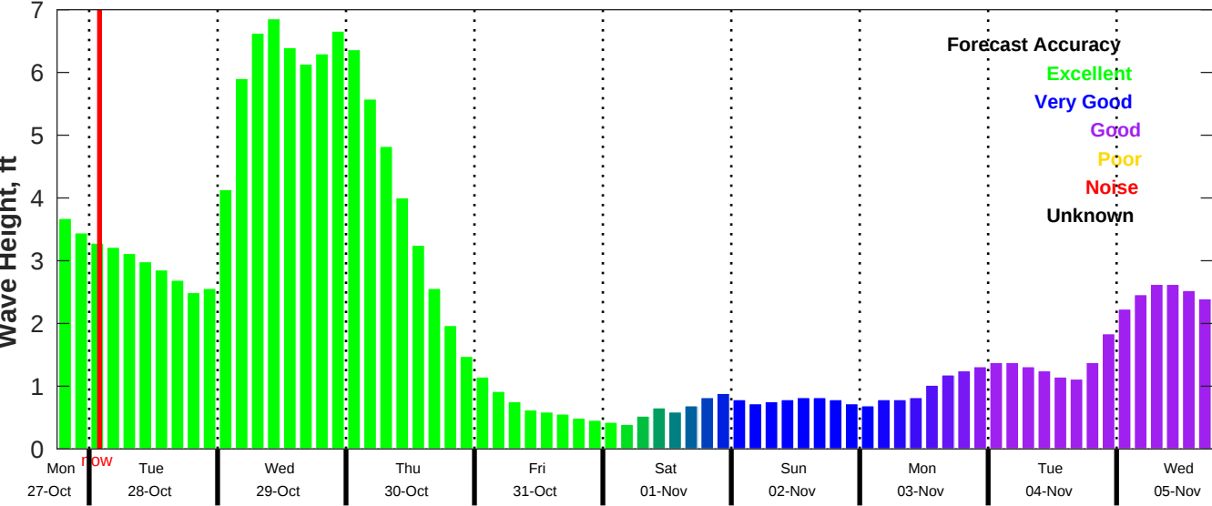
CMEMS Wave Forecast for NDBC 42019 from 27-Oct-2025 18:00:00 to 05-Nov-2025 18:00:00
