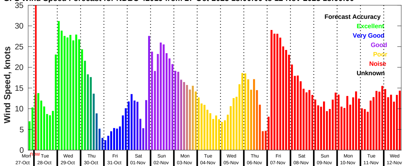
GFS Wind Speed Forecast for NDBC 42019 from 27-Oct-2025 18:00:00 to 12-Nov-2025 18:00:00
