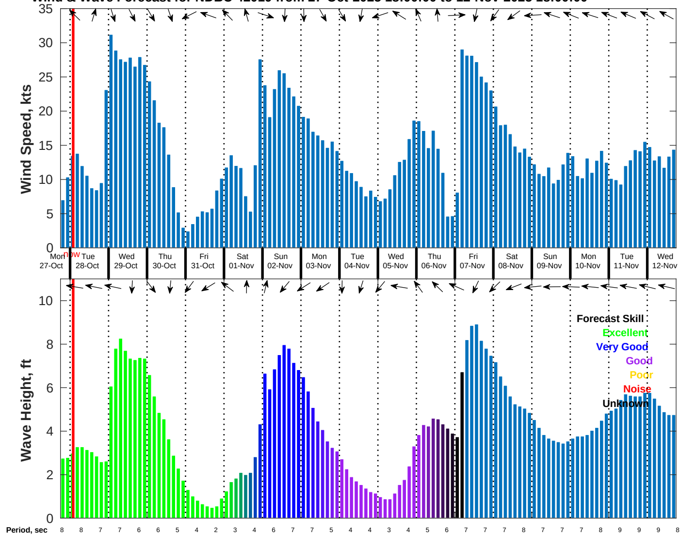
Wind & Wave Forecast for NDBC 42019 from 27-Oct-2025 18:00:00 to 12-Nov-2025 18:00:00
