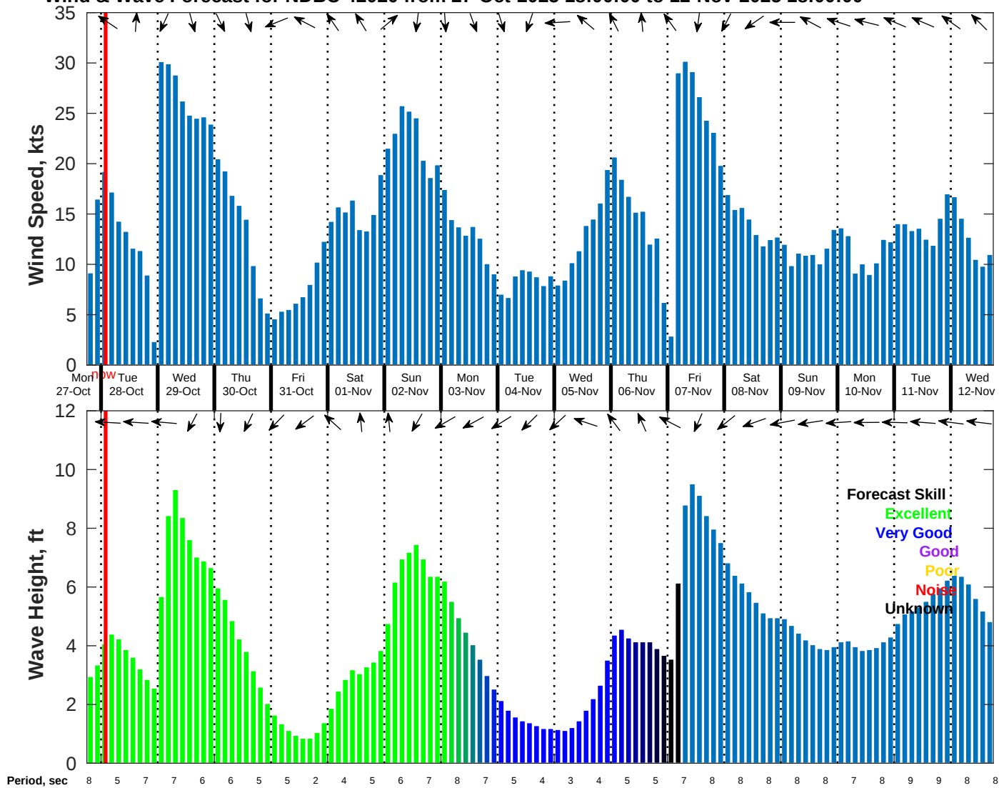
Wind & Wave Forecast for NDBC 42020 from 27-Oct-2025 18:00:00 to 12-Nov-2025 18:00:00
