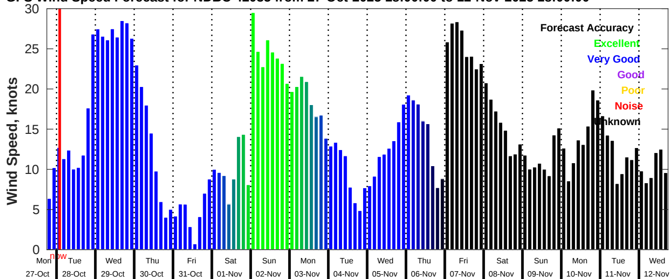
GFS Wind Speed Forecast for NDBC 42035 from 27-Oct-2025 18:00:00 to 12-Nov-2025 18:00:00
