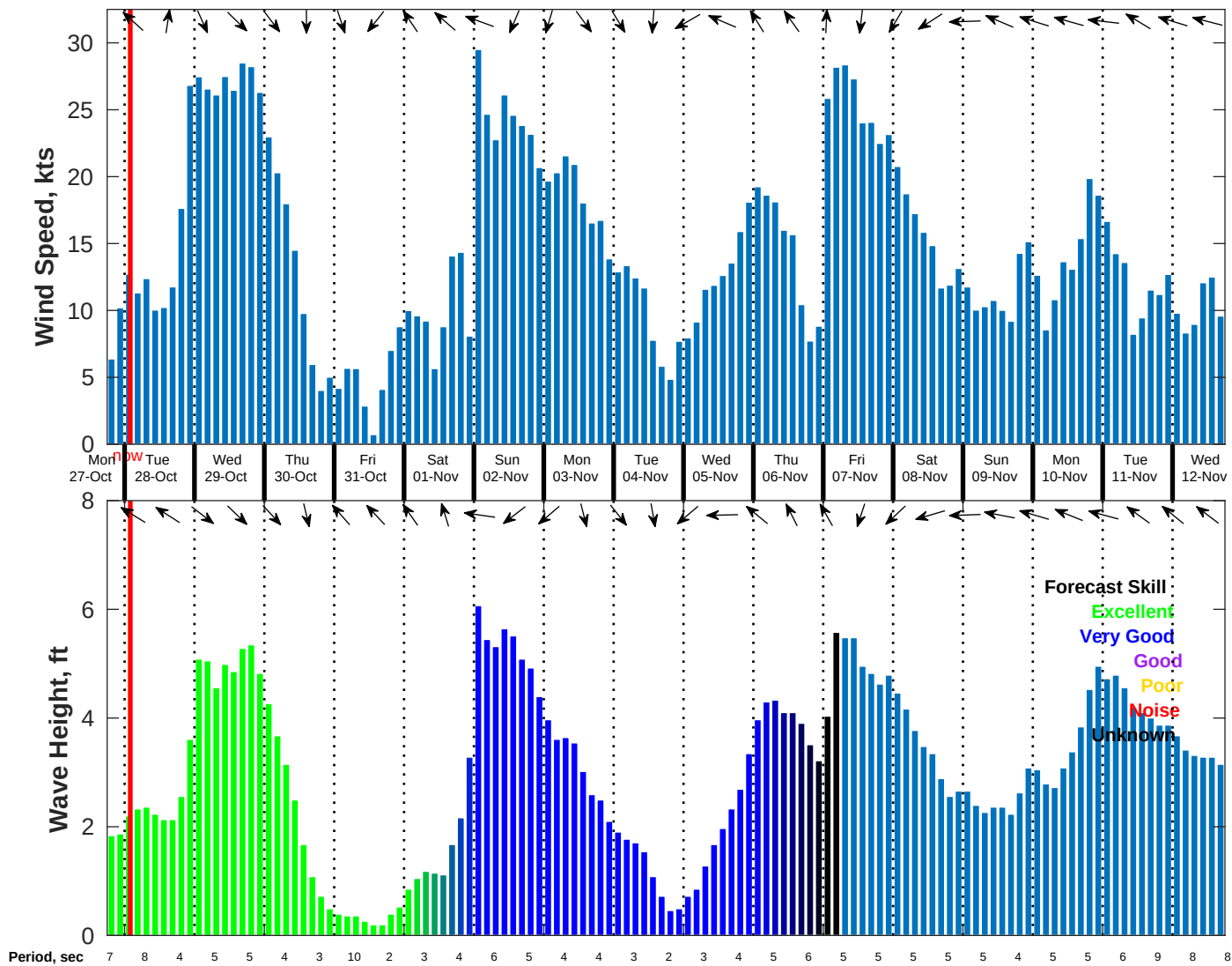
Wind & Wave Forecast for NDBC 42035 from 27-Oct-2025 18:00:00 to 12-Nov-2025 18:00:00
