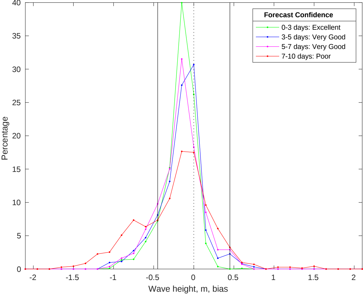
NDBC 42036 vs CMEMS Waves Bias Histogram: 28-Oct-2025
