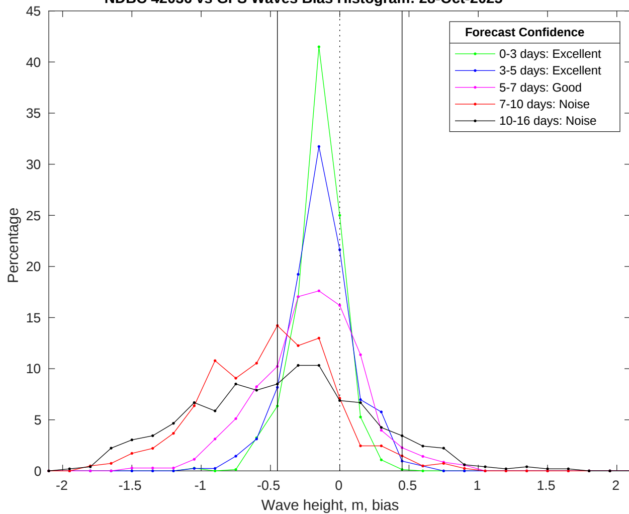
NDBC 42036 vs GFS Waves Bias Histogram: 28-Oct-2025
