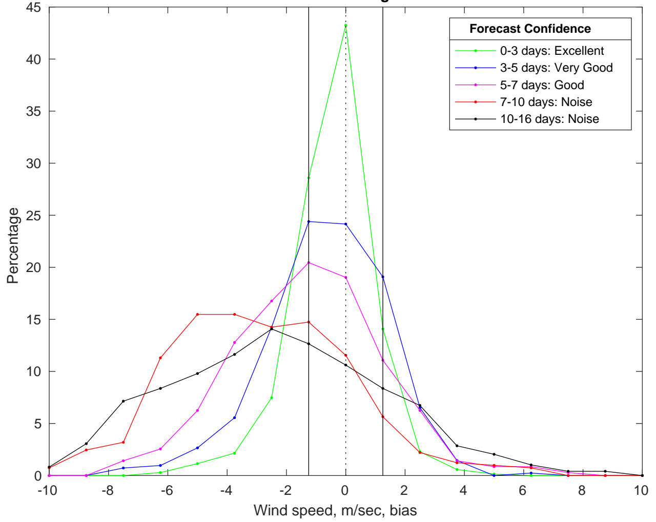
NDBC 42036 vs GFS Winds Bias Histogram: 28-Oct-2025
