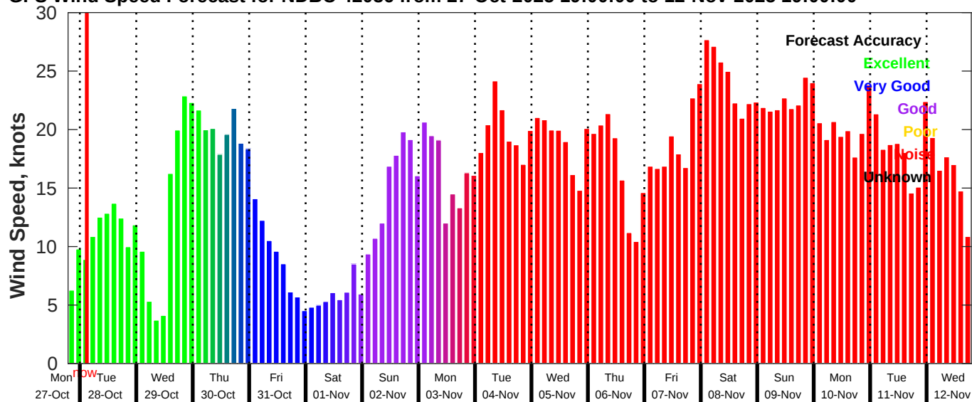
GFS Wind Speed Forecast for NDBC 42036 from 27-Oct-2025 19:00:00 to 12-Nov-2025 19:00:00
