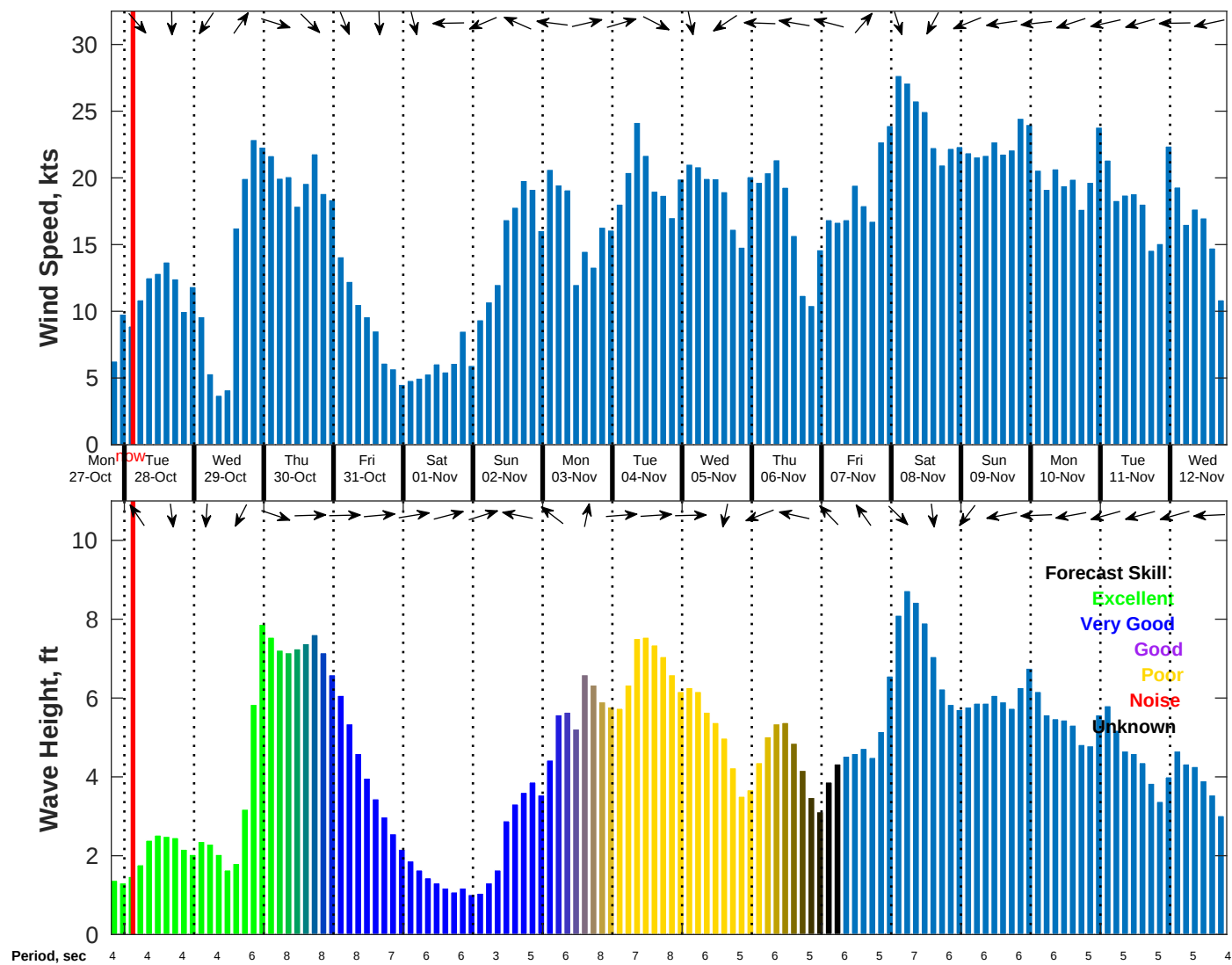
Wind & Wave Forecast for NDBC 42036 from 27-Oct-2025 19:00:00 to 12-Nov-2025 19:00:00
