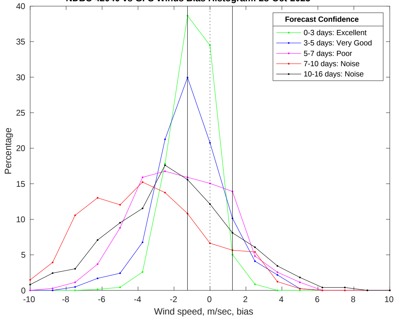
NDBC 42040 vs GFS Winds Bias Histogram: 28-Oct-2025
