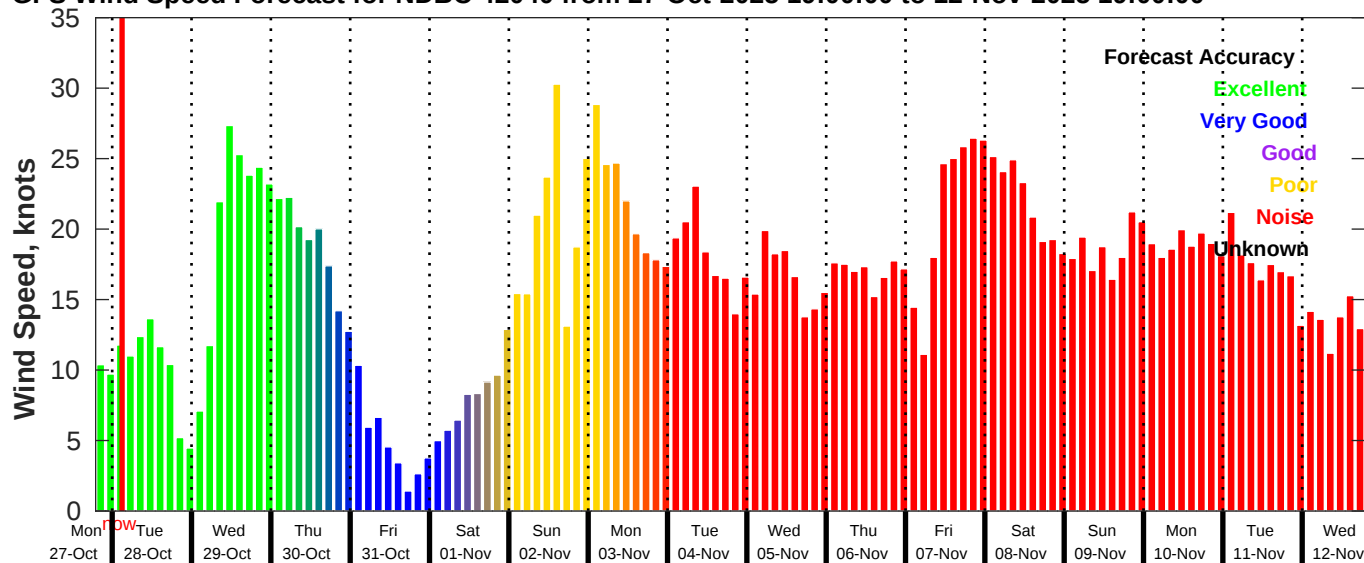
GFS Wind Speed Forecast for NDBC 42040 from 27-Oct-2025 19:00:00 to 12-Nov-2025 19:00:00
