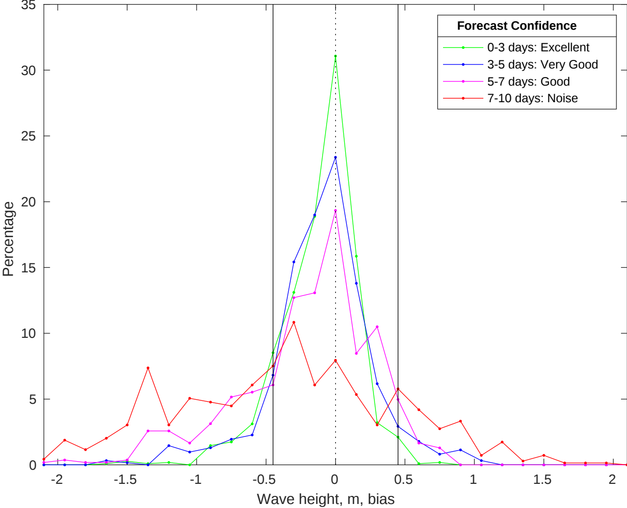
NDBC 44008 vs CMEMS Waves Bias Histogram: 28-Oct-2025
