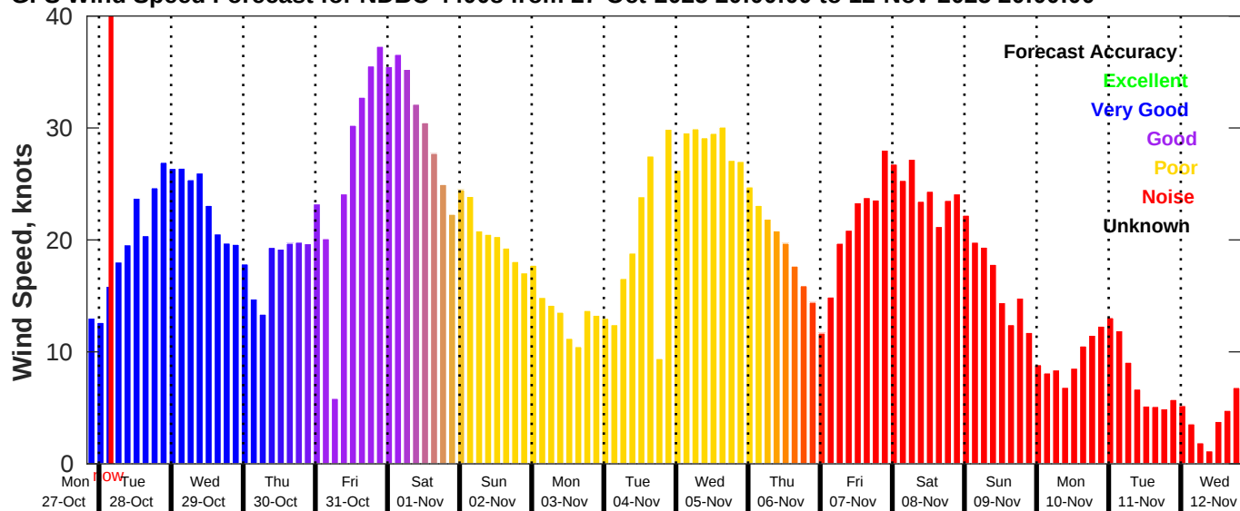
GFS Wind Speed Forecast for NDBC 44008 from 27-Oct-2025 20:00:00 to 12-Nov-2025 20:00:00
