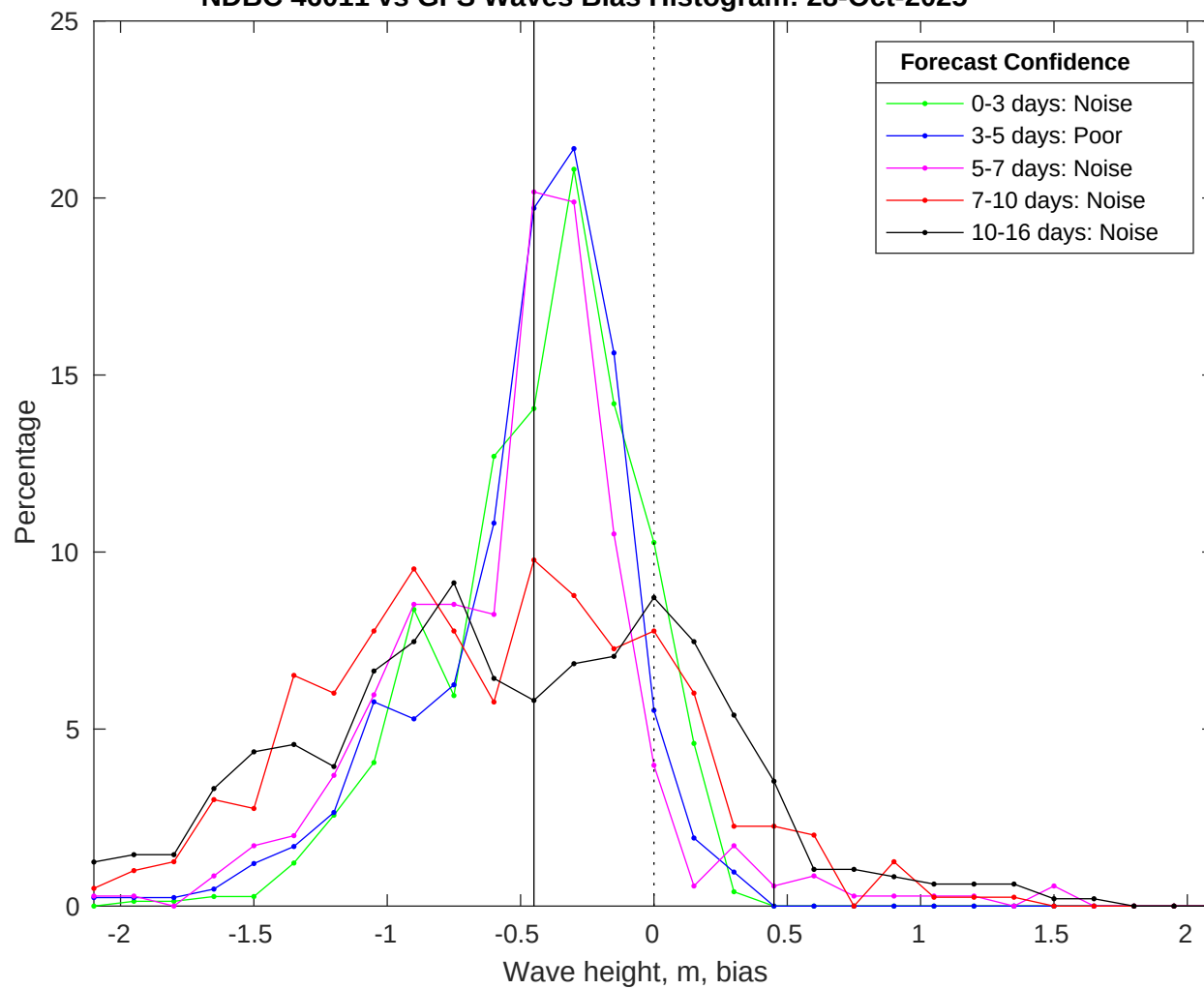
NDBC 46011 vs GFS Waves Bias Histogram: 28-Oct-2025
