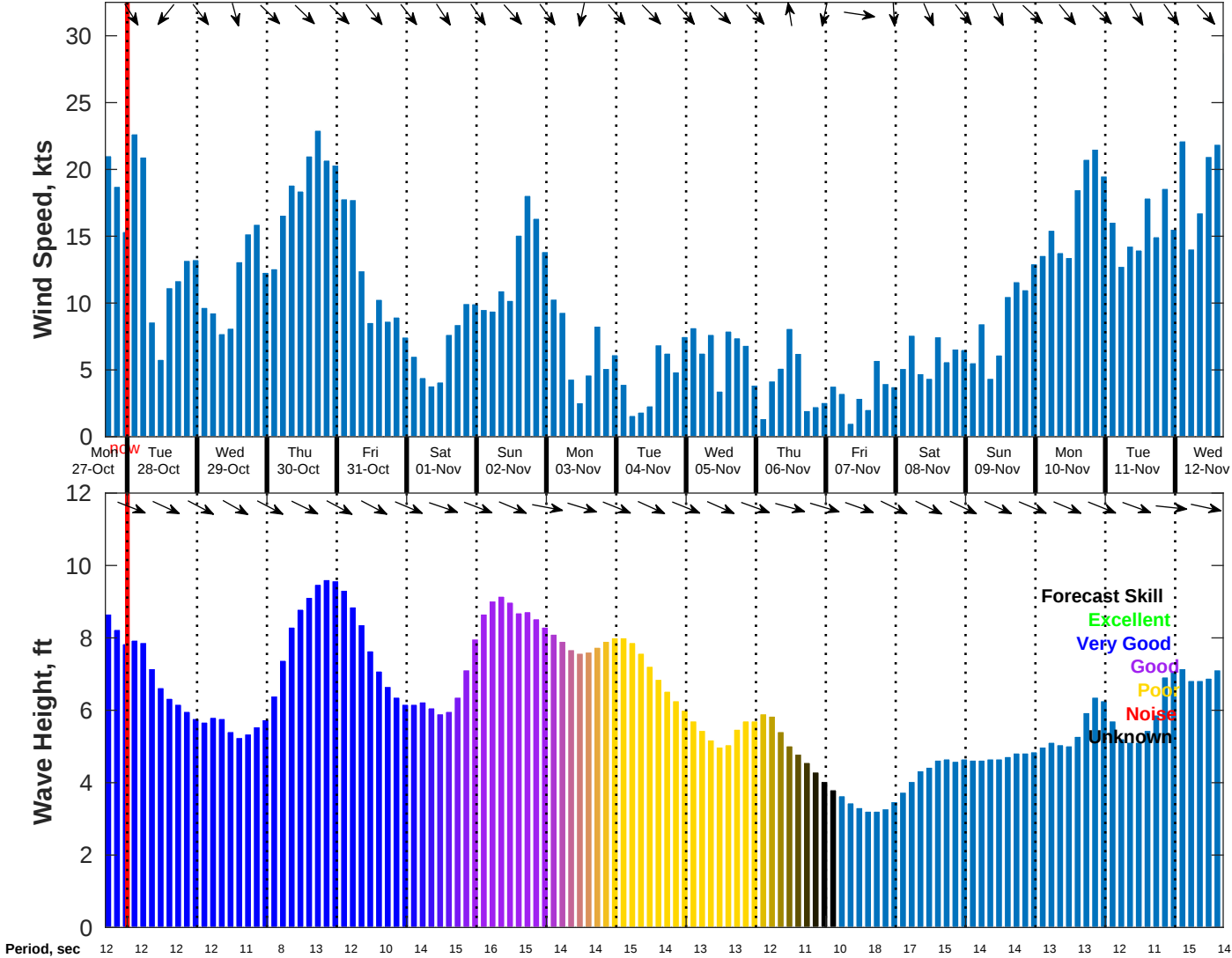
Wind & Wave Forecast for NDBC 46011 from 27-Oct-2025 16:00:00 to 12-Nov-2025 16:00:00
