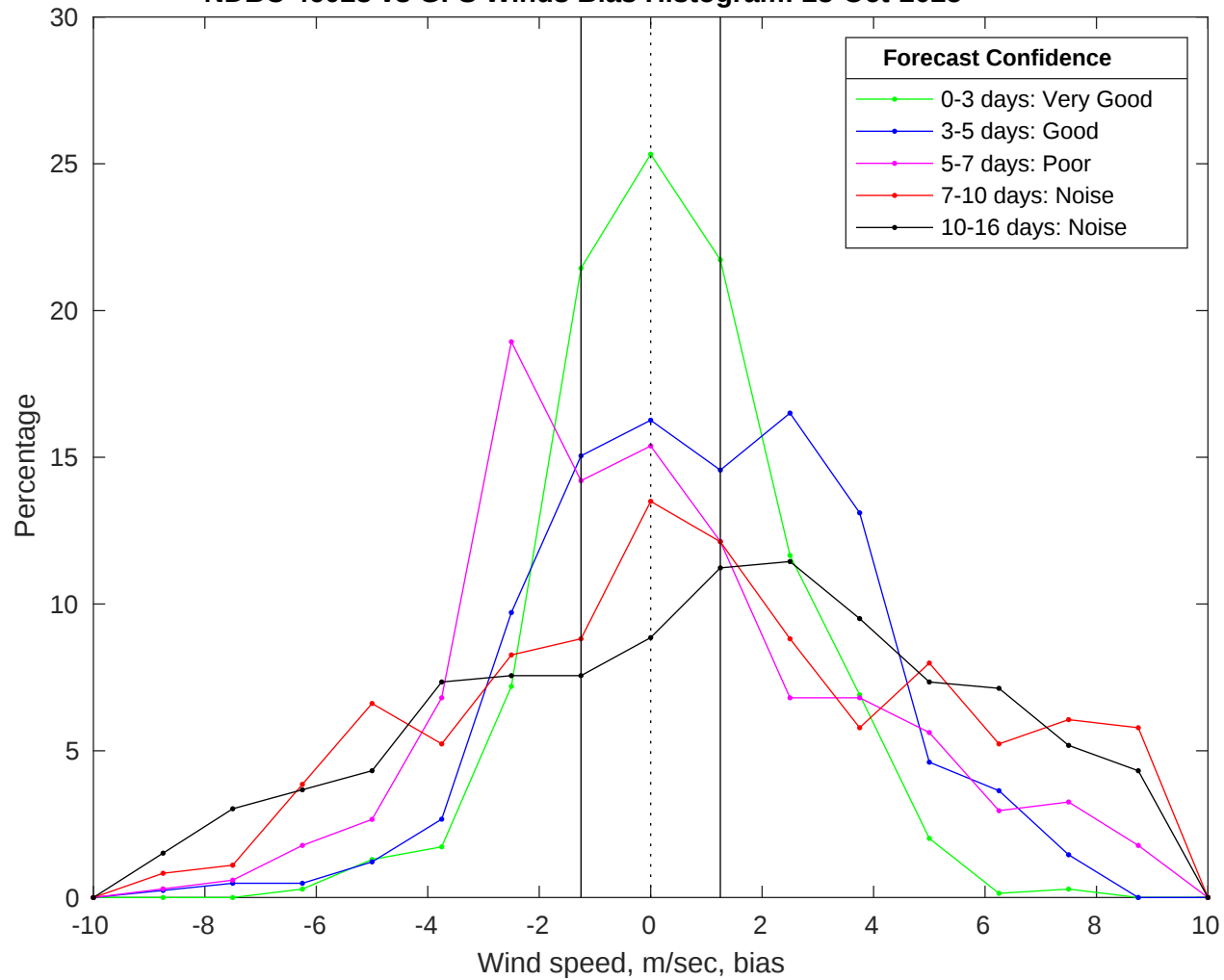
NDBC 46028 vs GFS Winds Bias Histogram: 28-Oct-2025
