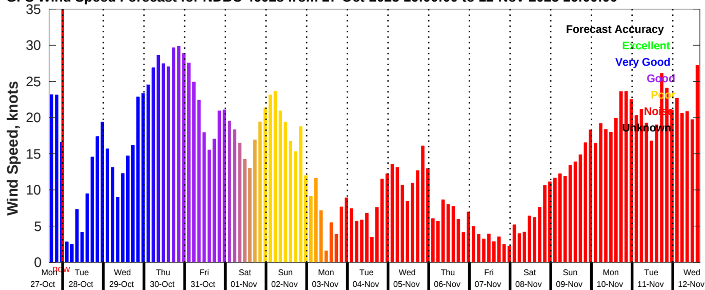
GFS Wind Speed Forecast for NDBC 46028 from 27-Oct-2025 16:00:00 to 12-Nov-2025 16:00:00
