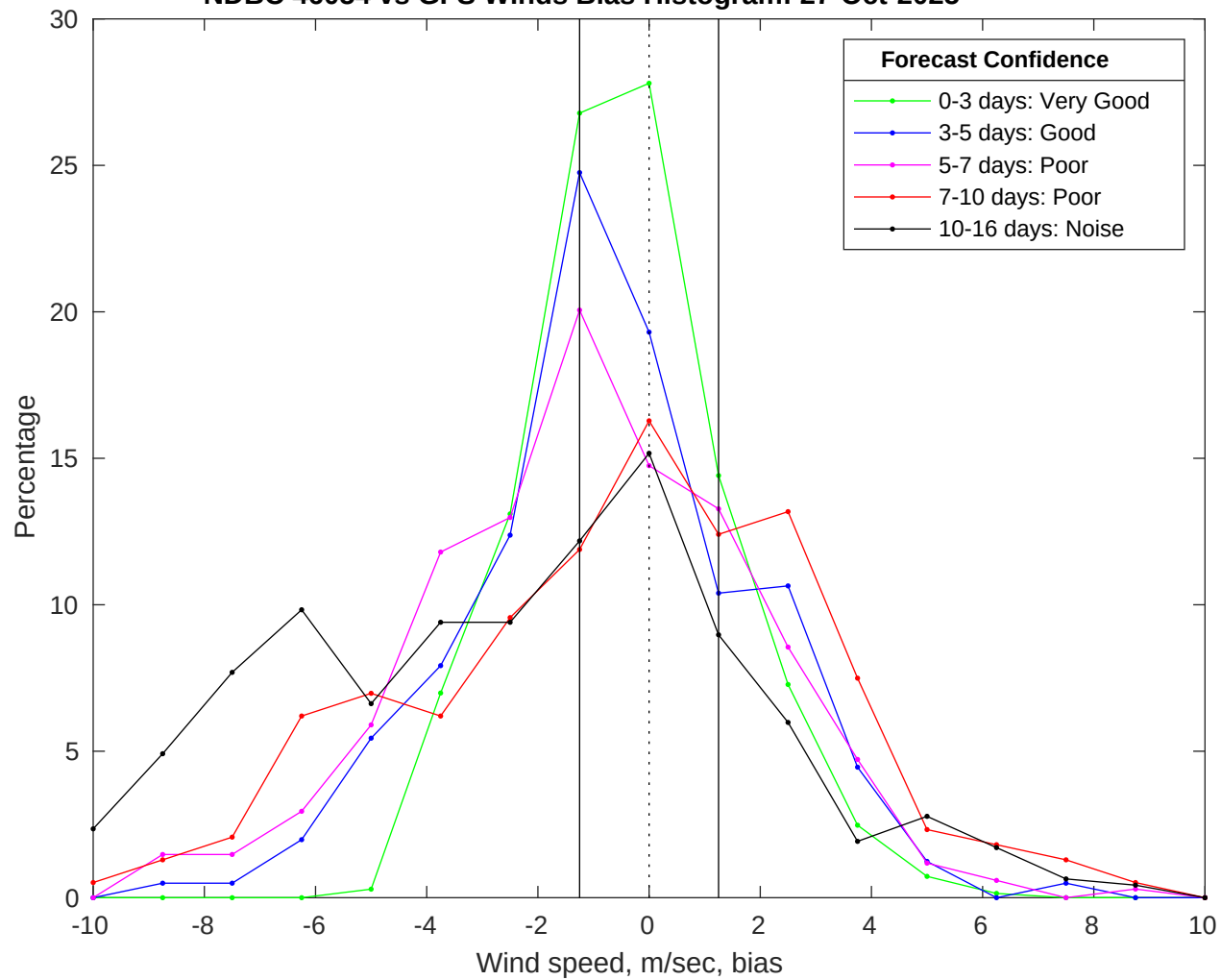
NDBC 46054 vs GFS Winds Bias Histogram: 27-Oct-2025
