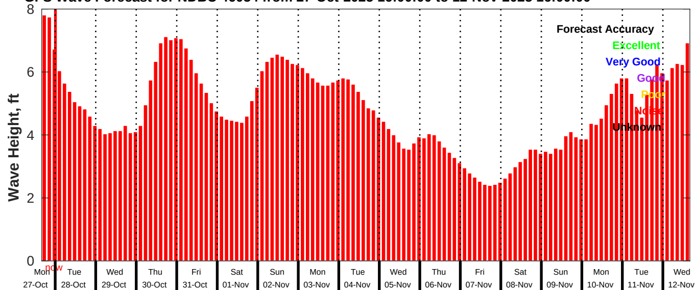
GFS Wave Forecast for NDBC 46054 from 27-Oct-2025 16:00:00 to 12-Nov-2025 16:00:00
