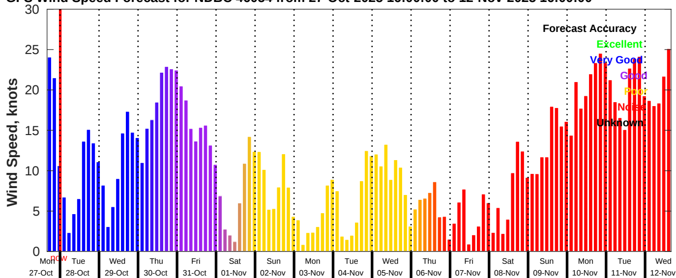
GFS Wind Speed Forecast for NDBC 46054 from 27-Oct-2025 16:00:00 to 12-Nov-2025 16:00:00
