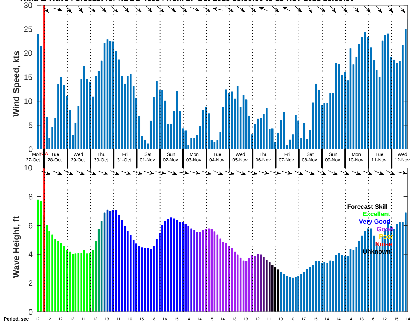
Wind & Wave Forecast for NDBC 46054 from 27-Oct-2025 16:00:00 to 12-Nov-2025 16:00:00
