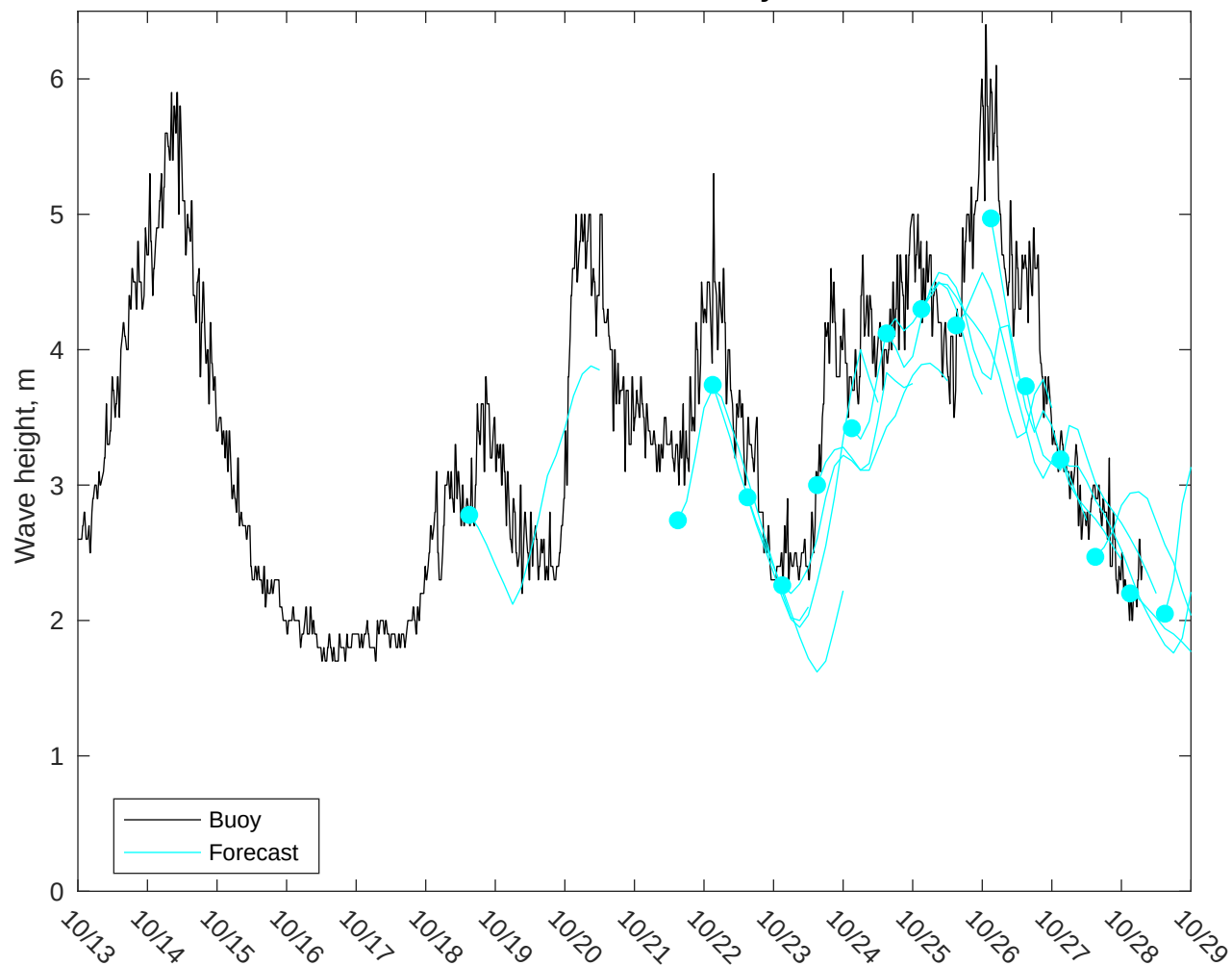
NDBC 46059 vs GFS Waves: 5 to 7 day forecast
