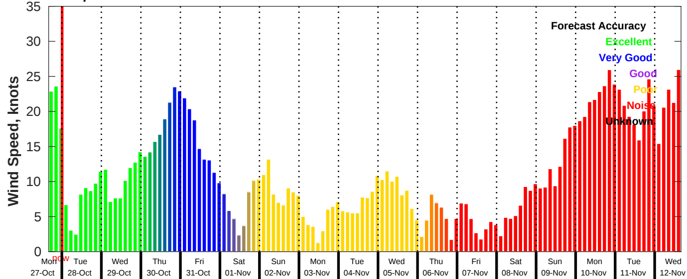
GFS Wind Speed Forecast for NDBC 46069 from 27-Oct-2025 16:00:00 to 12-Nov-2025 16:00:00
