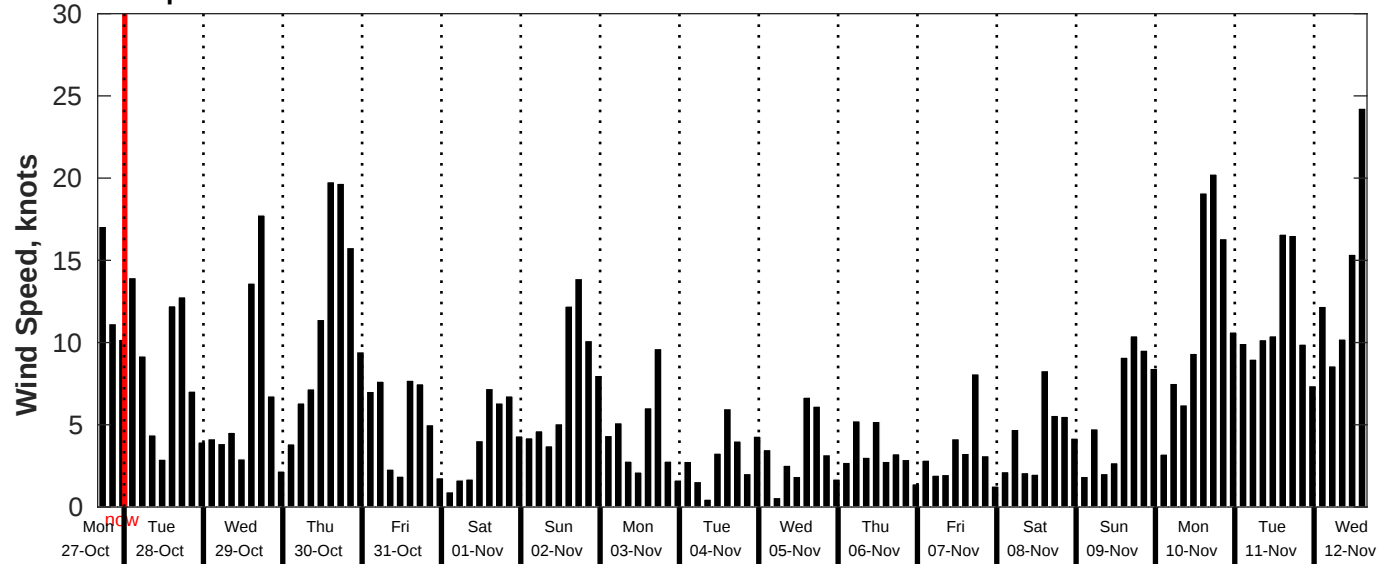
GFS Wind Speed Forecast for NDBC 46215 from 27-Oct-2025 16:00:00 to 12-Nov-2025 16:00:00
