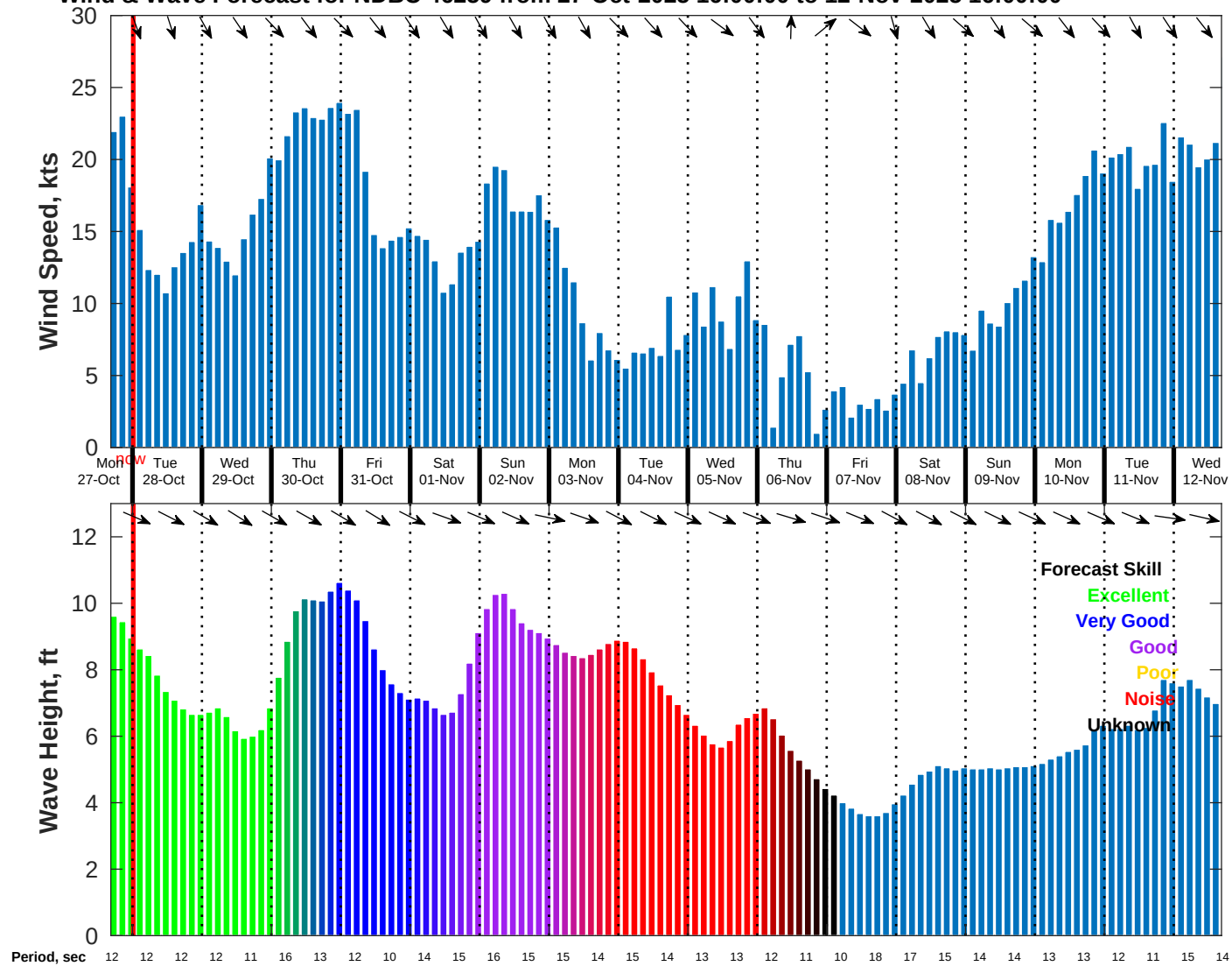
Wind & Wave Forecast for NDBC 46259 from 27-Oct-2025 16:00:00 to 12-Nov-2025 16:00:00
