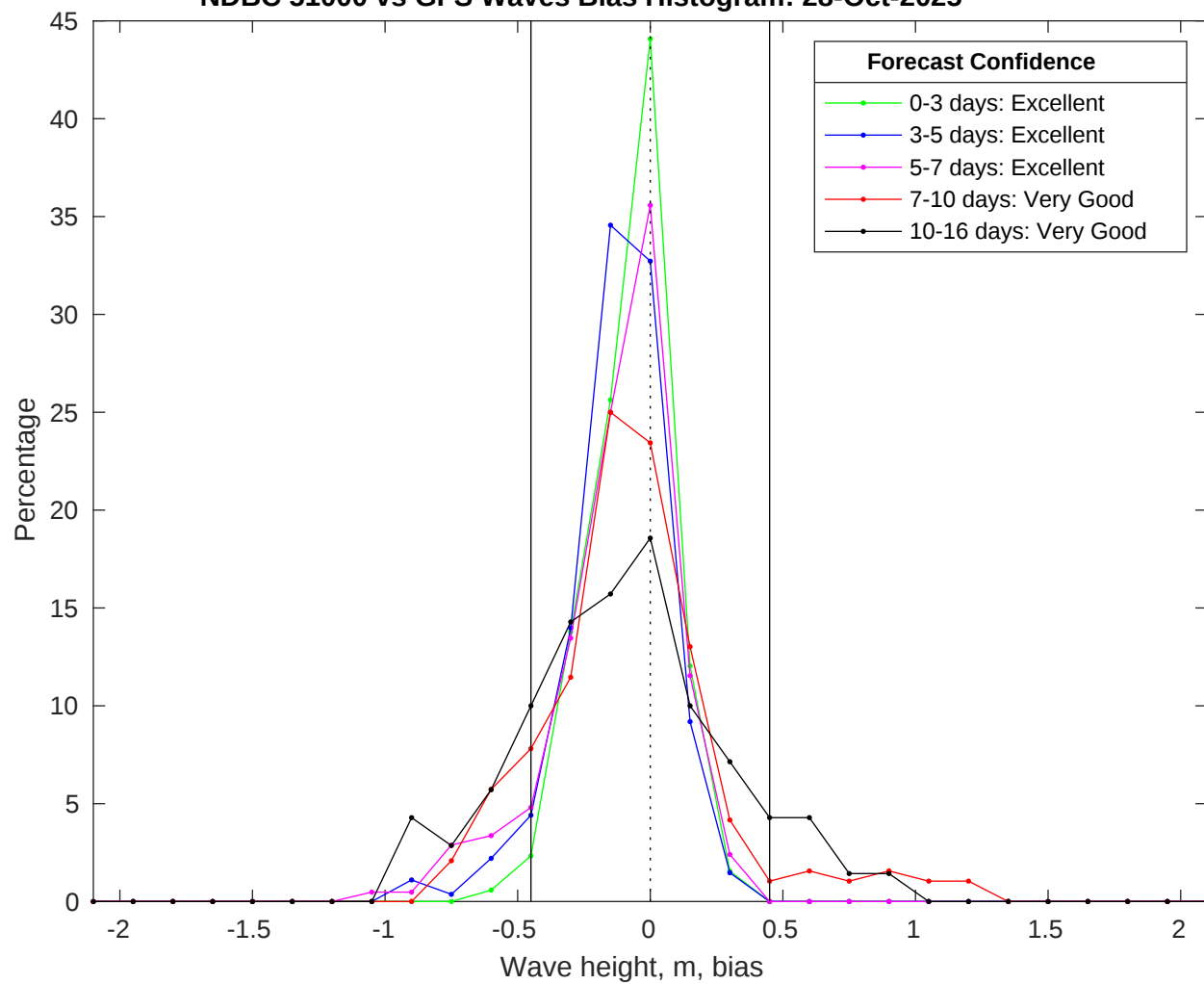
NDBC 51000 vs GFS Waves Bias Histogram: 28-Oct-2025
