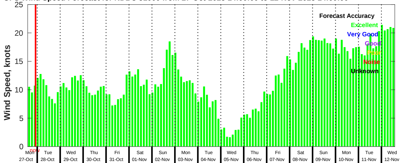
GFS Wind Speed Forecast for NDBC 51000 from 27-Oct-2025 14:00:00 to 12-Nov-2025 14:00:00
