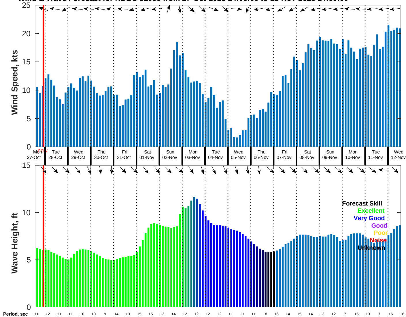
Wind & Wave Forecast for NDBC 51000 from 27-Oct-2025 14:00:00 to 12-Nov-2025 14:00:00
