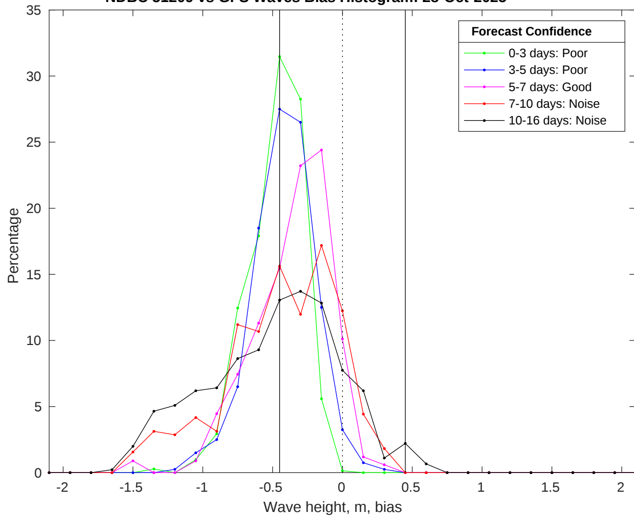
NDBC 51209 vs GFS Waves Bias Histogram: 28-Oct-2025
