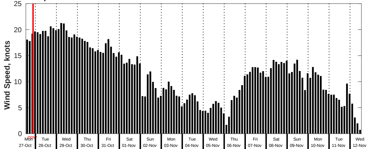
GFS Wind Speed Forecast for NDBC 51209 from 27-Oct-2025 13:00:00 to 12-Nov-2025 13:00:00
