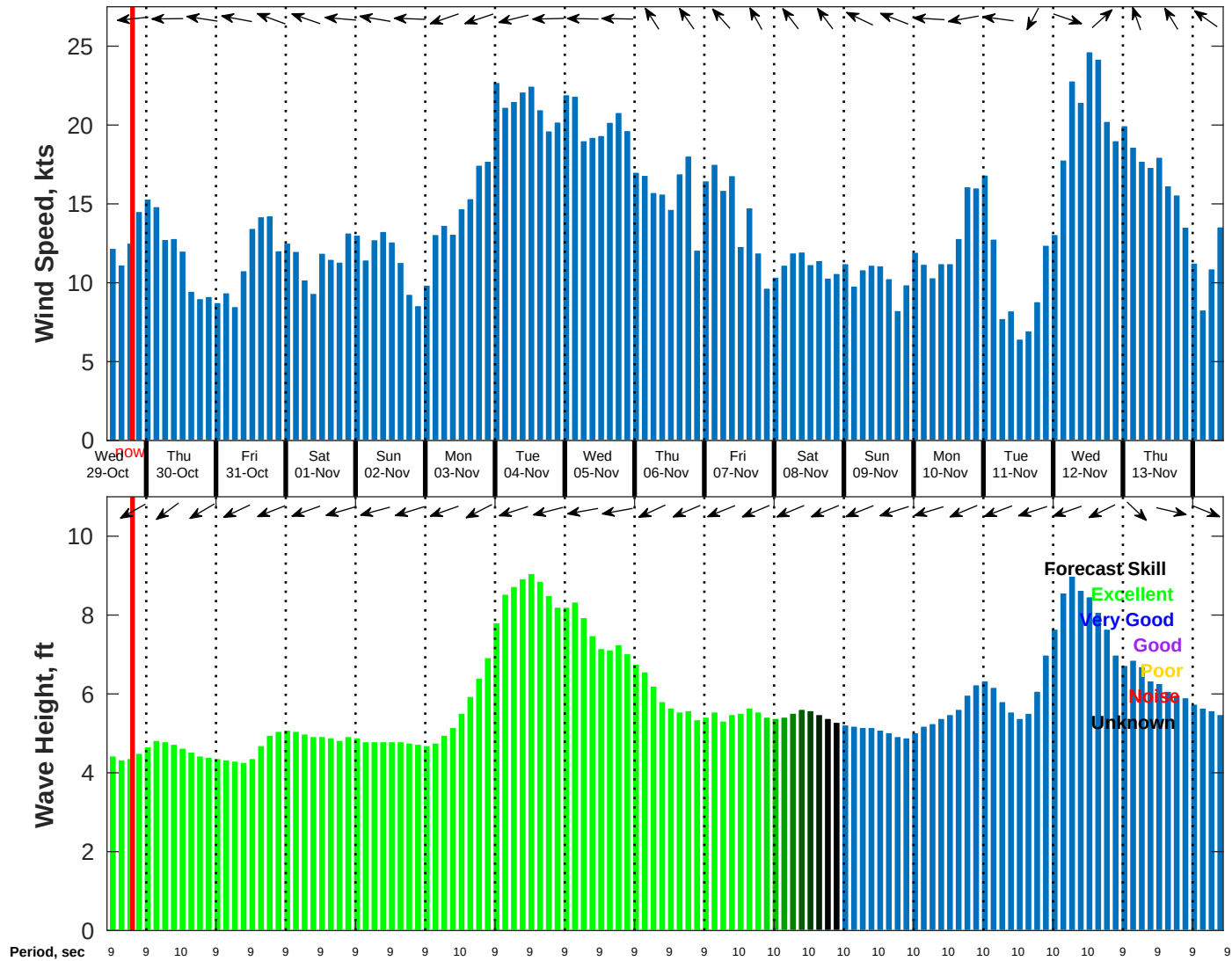
Wind & Wave Forecast for NDBC 52211 from 28-Oct-2025 11:00:00 to 13-Nov-2025 11:00:00
