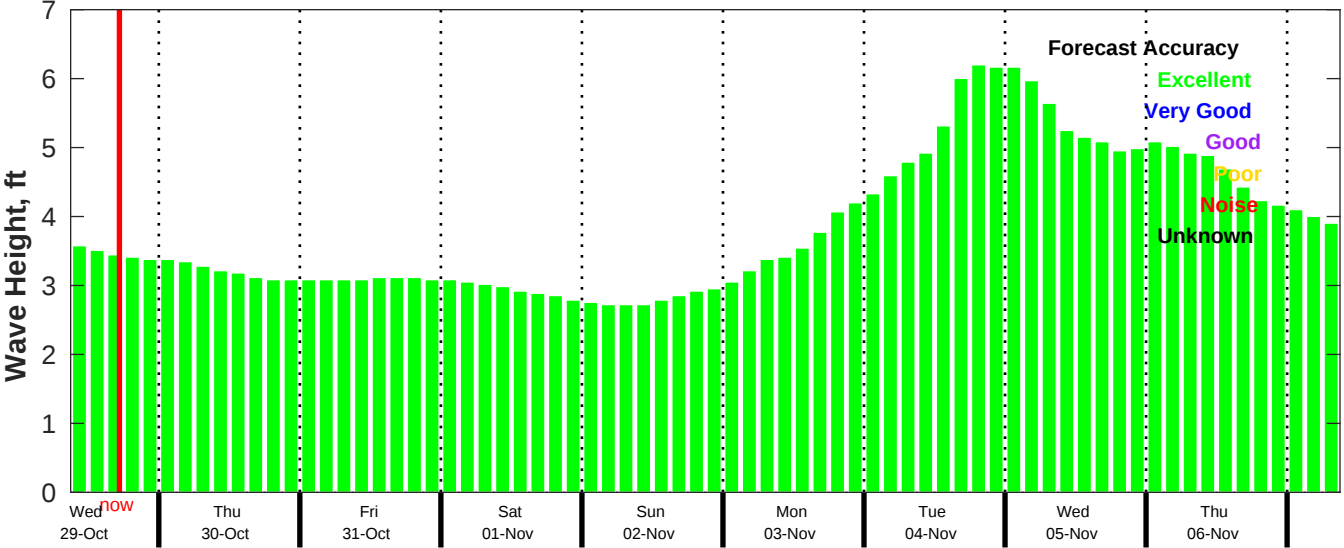
CMEMS Wave Forecast for NDBC 52212 from 28-Oct-2025 09:00:00 to 06-Nov-2025 09:00:00
