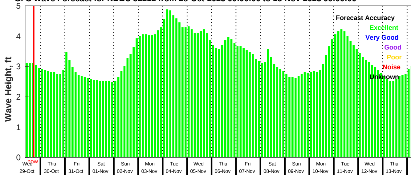
GFS Wave Forecast for NDBC 52212 from 28-Oct-2025 09:00:00 to 13-Nov-2025 09:00:00
