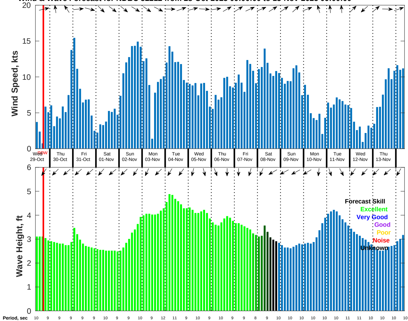
Wind & Wave Forecast for NDBC 52212 from 28-Oct-2025 09:00:00 to 13-Nov-2025 09:00:00
