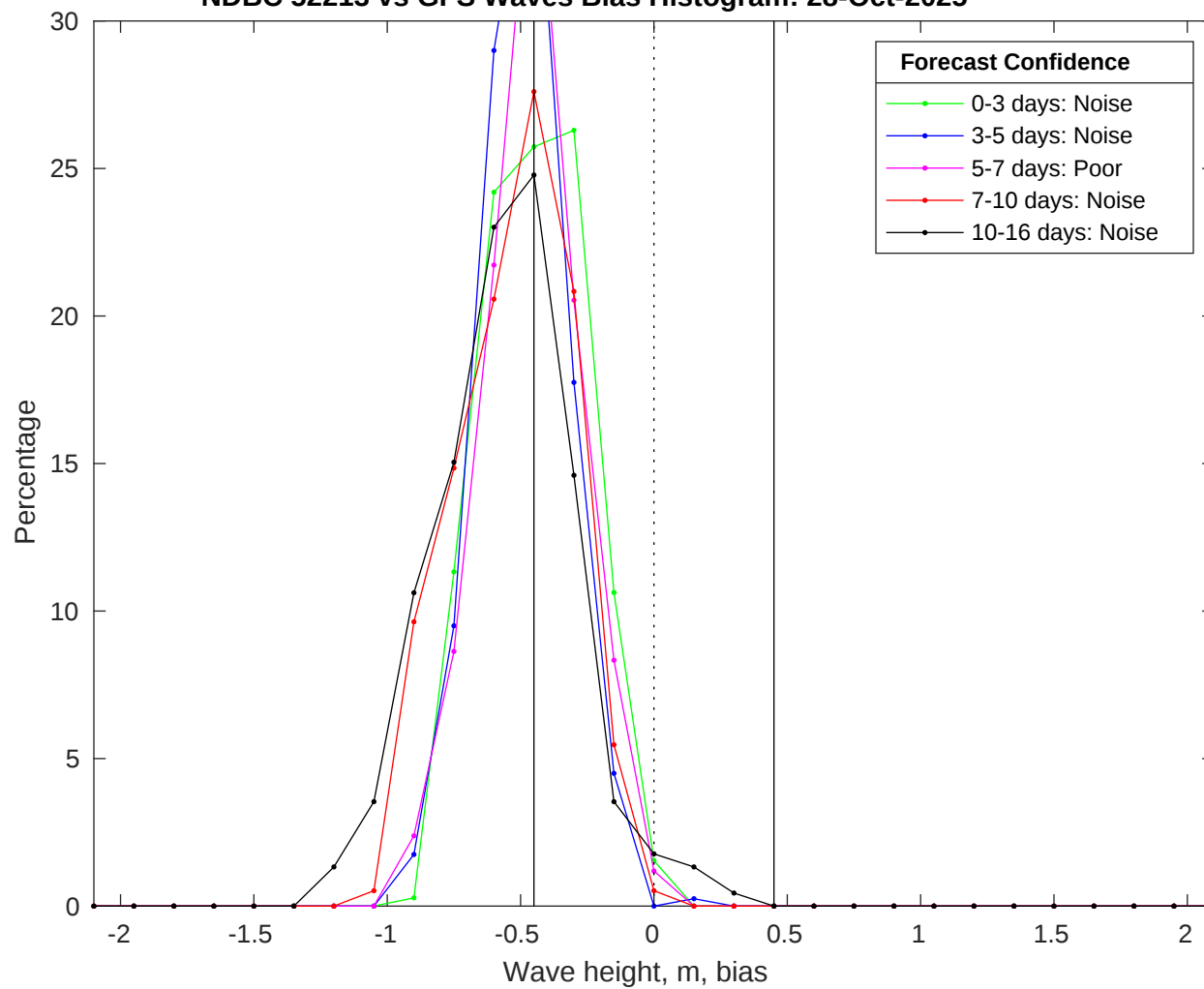
NDBC 52213 vs GFS Waves Bias Histogram: 28-Oct-2025
