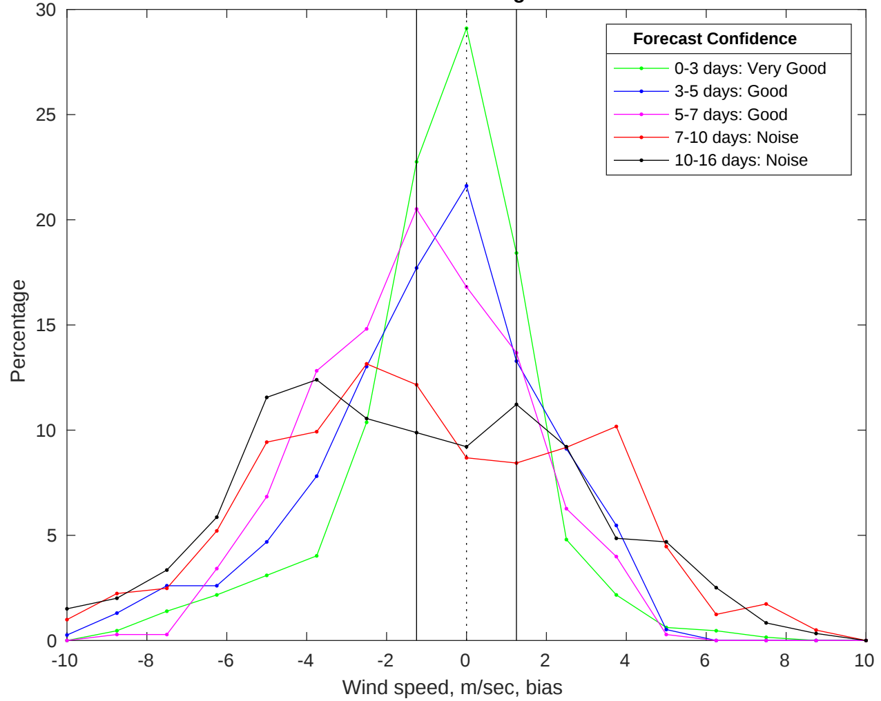
NDBC 41004 vs GFS Winds Bias Histogram: 29-Oct-2025
