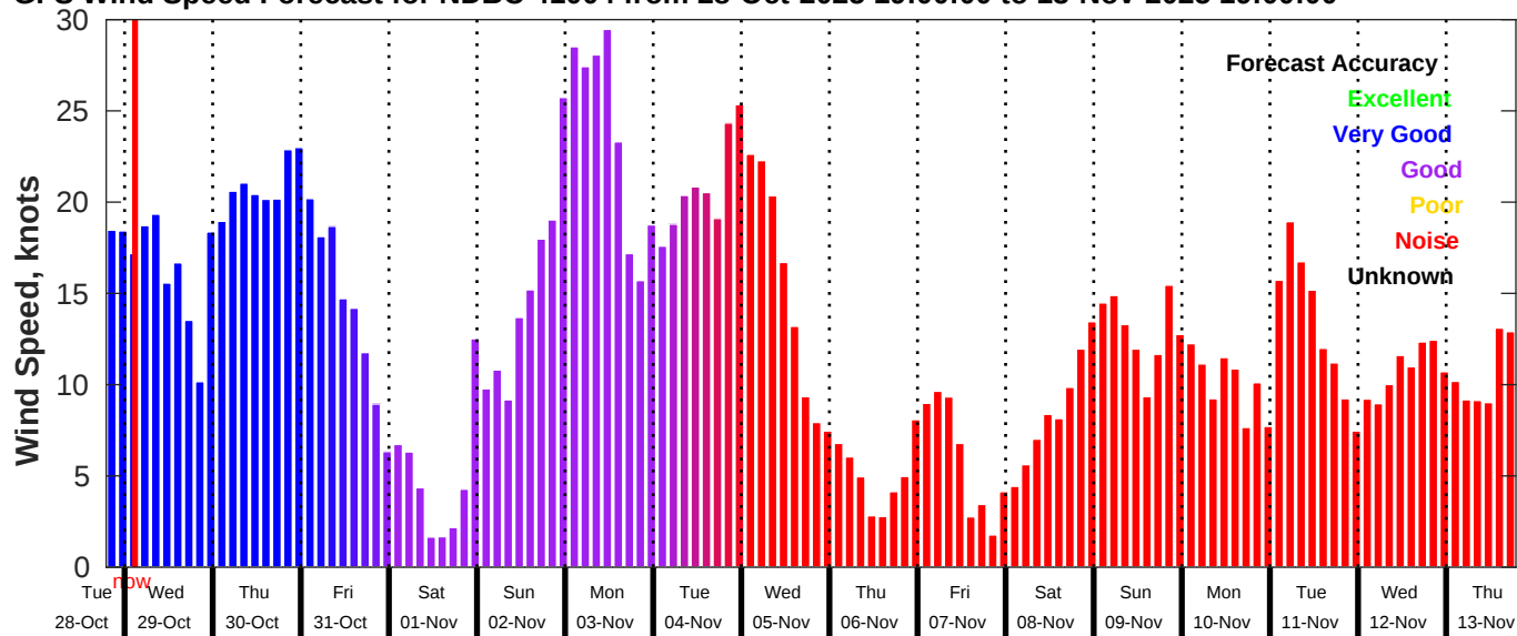
GFS Wind Speed Forecast for NDBC 41004 from 28-Oct-2025 19:00:00 to 13-Nov-2025 19:00:00
