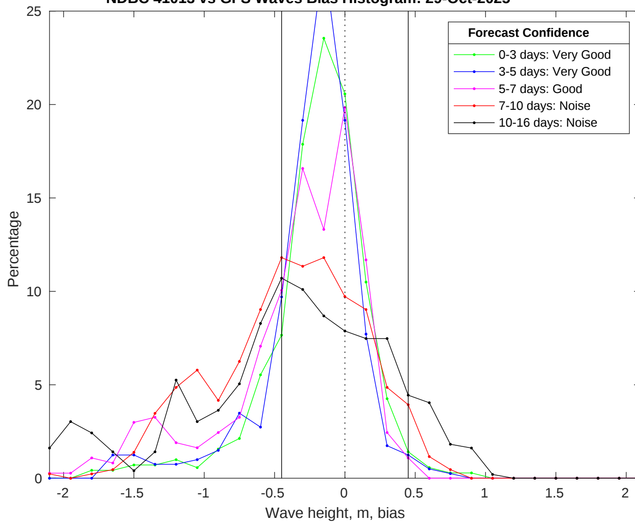
NDBC 41013 vs GFS Waves Bias Histogram: 29-Oct-2025
