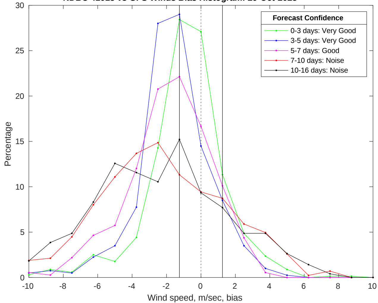
NDBC 41013 vs GFS Winds Bias Histogram: 29-Oct-2025
