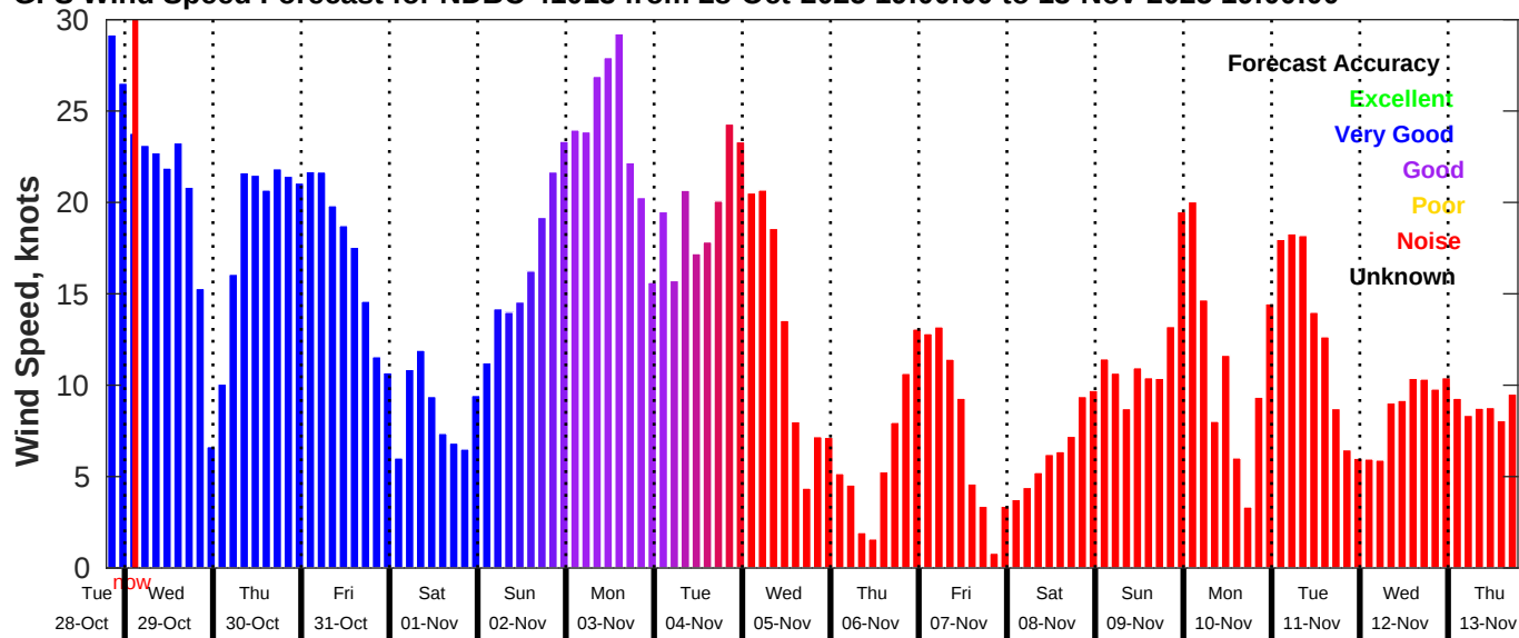
GFS Wind Speed Forecast for NDBC 41013 from 28-Oct-2025 19:00:00 to 13-Nov-2025 19:00:00
