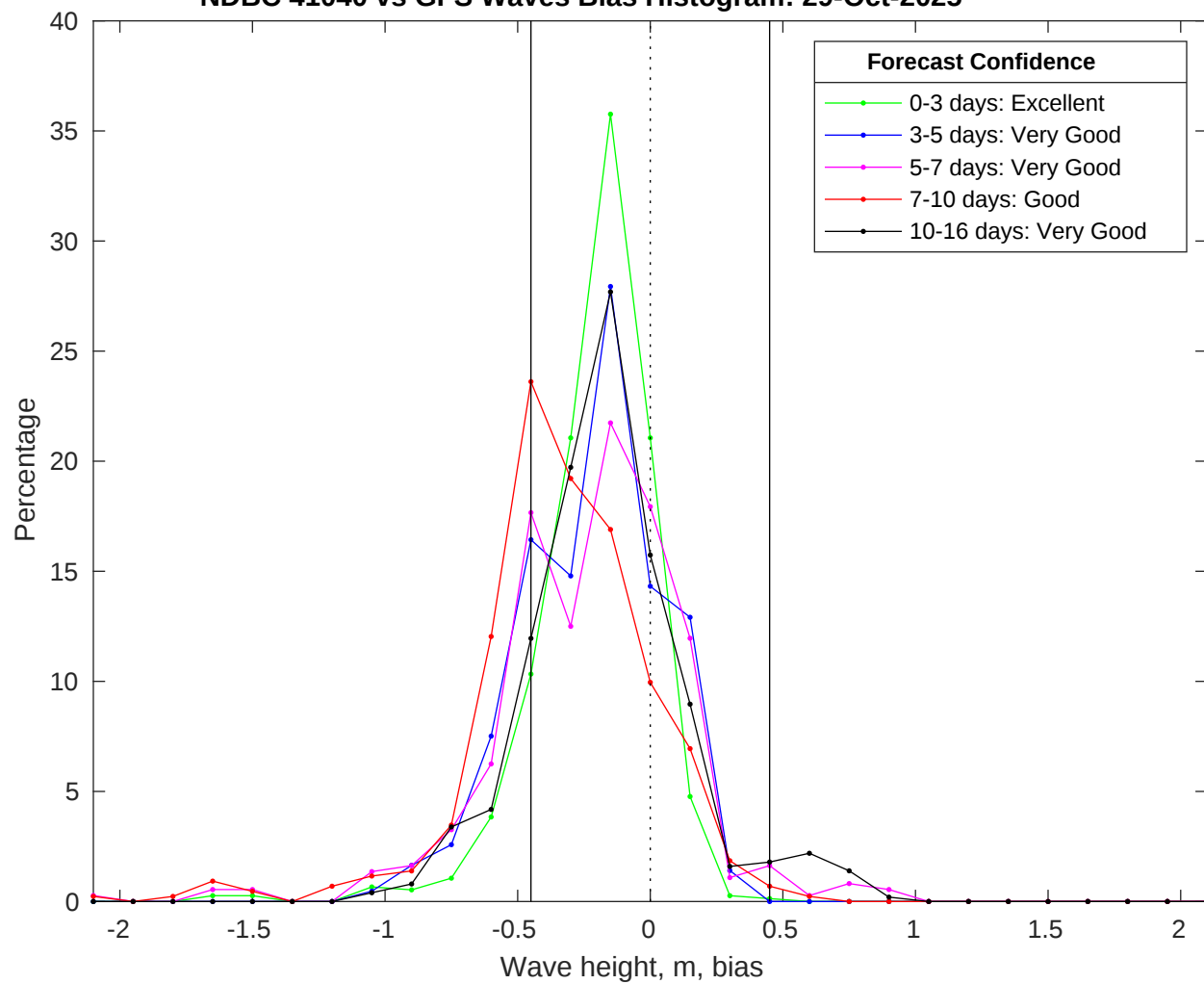
NDBC 41040 vs GFS Waves Bias Histogram: 29-Oct-2025
