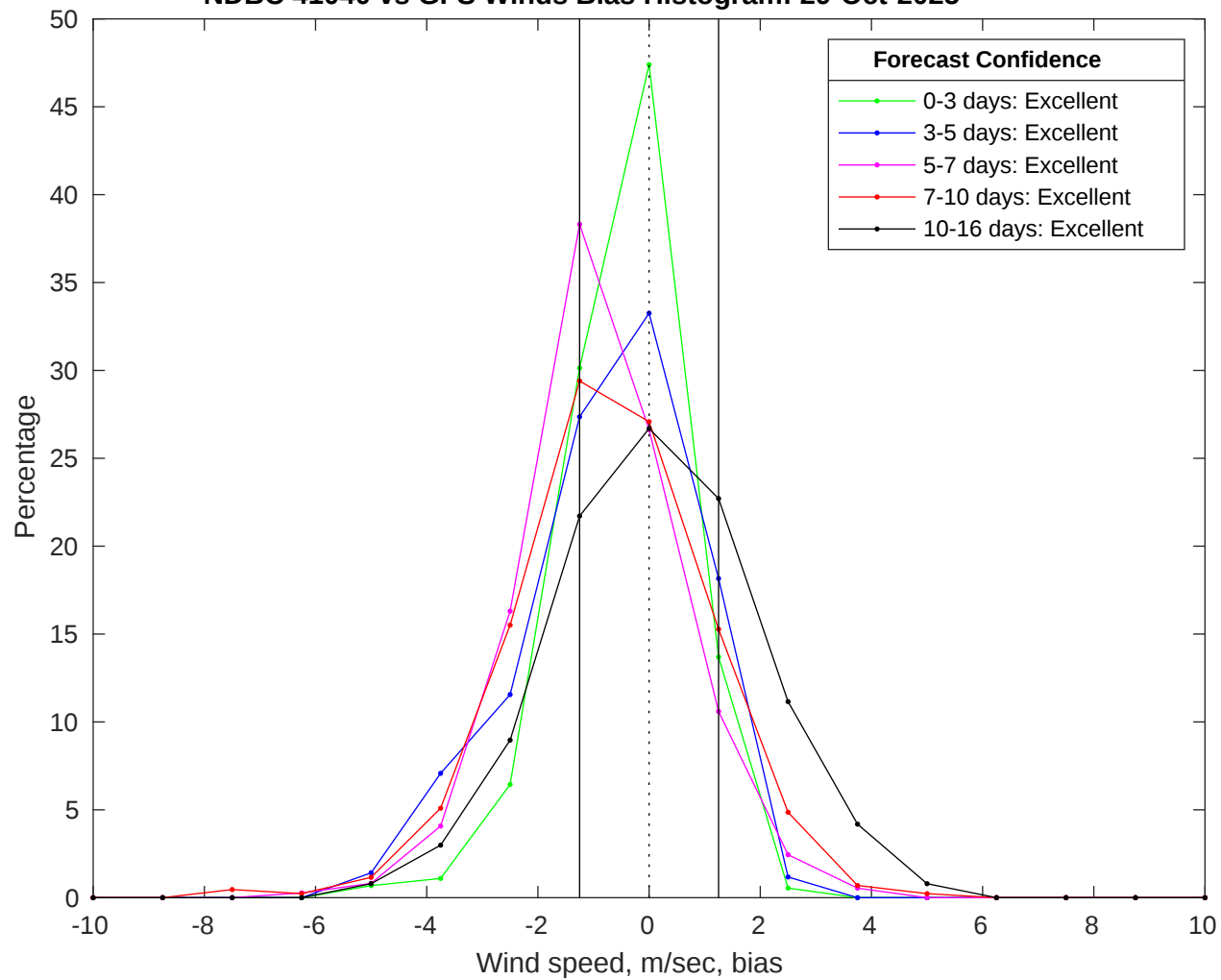
NDBC 41040 vs GFS Winds Bias Histogram: 29-Oct-2025
