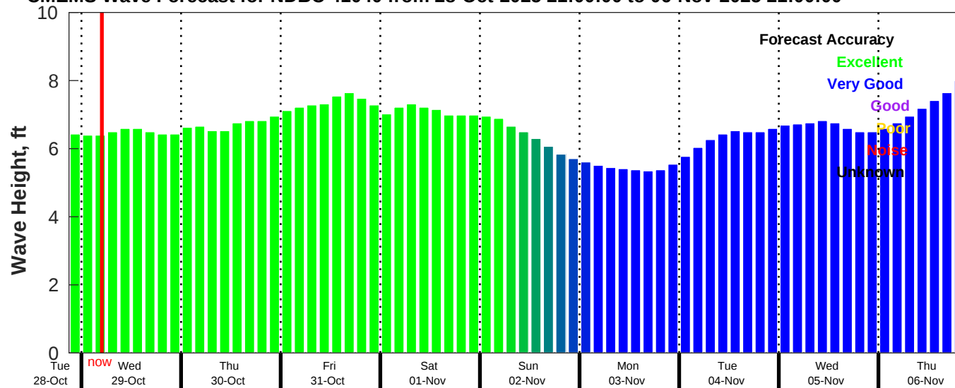
CMEMS Wave Forecast for NDBC 41040 from 28-Oct-2025 21:00:00 to 06-Nov-2025 21:00:00
