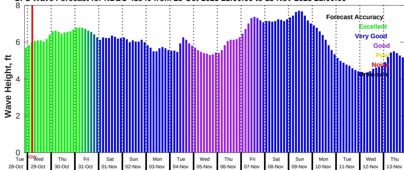
GFS Wave Forecast for NDBC 41040 from 28-Oct-2025 21:00:00 to 13-Nov-2025 21:00:00
