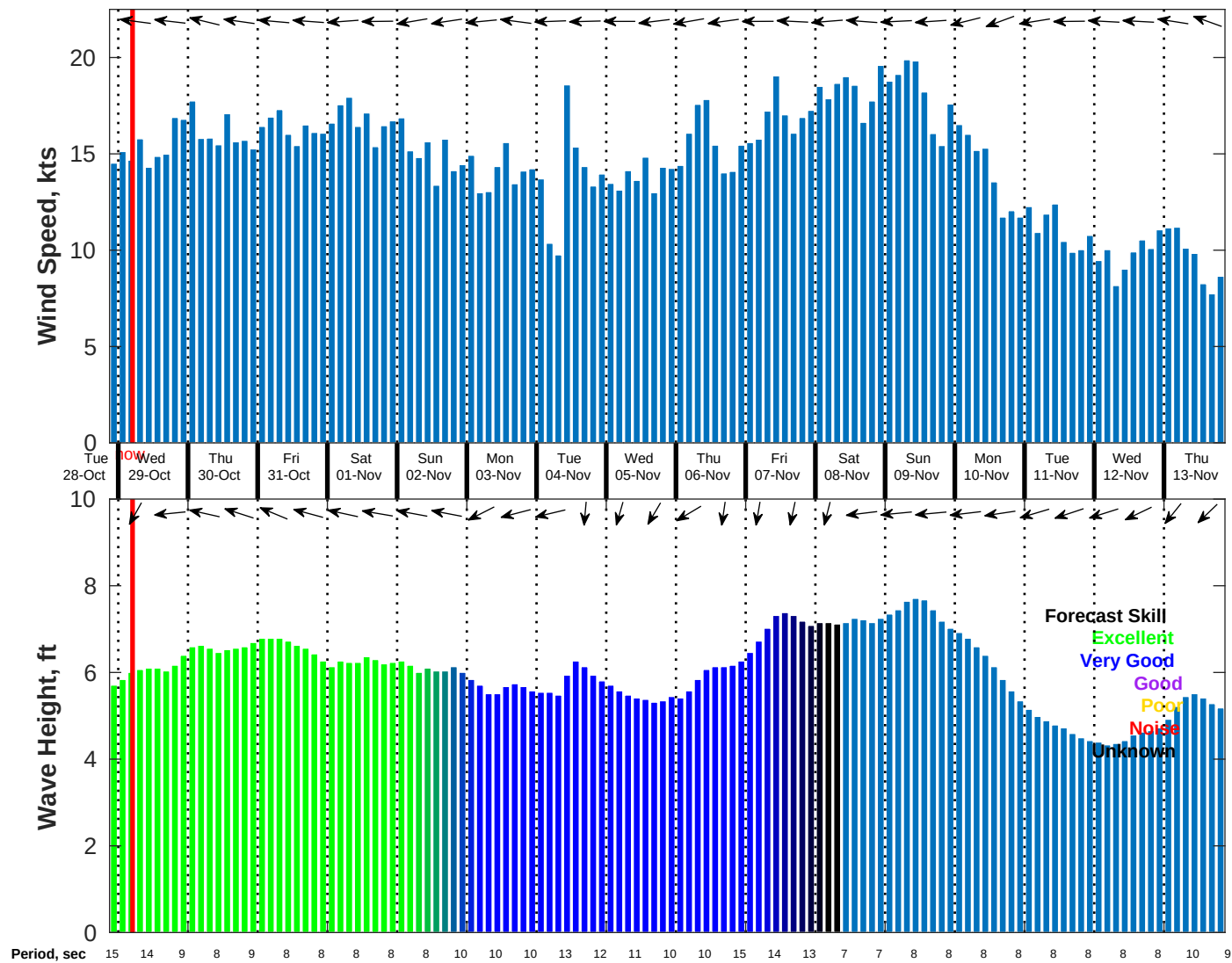
Wind & Wave Forecast for NDBC 41040 from 28-Oct-2025 21:00:00 to 13-Nov-2025 21:00:00
