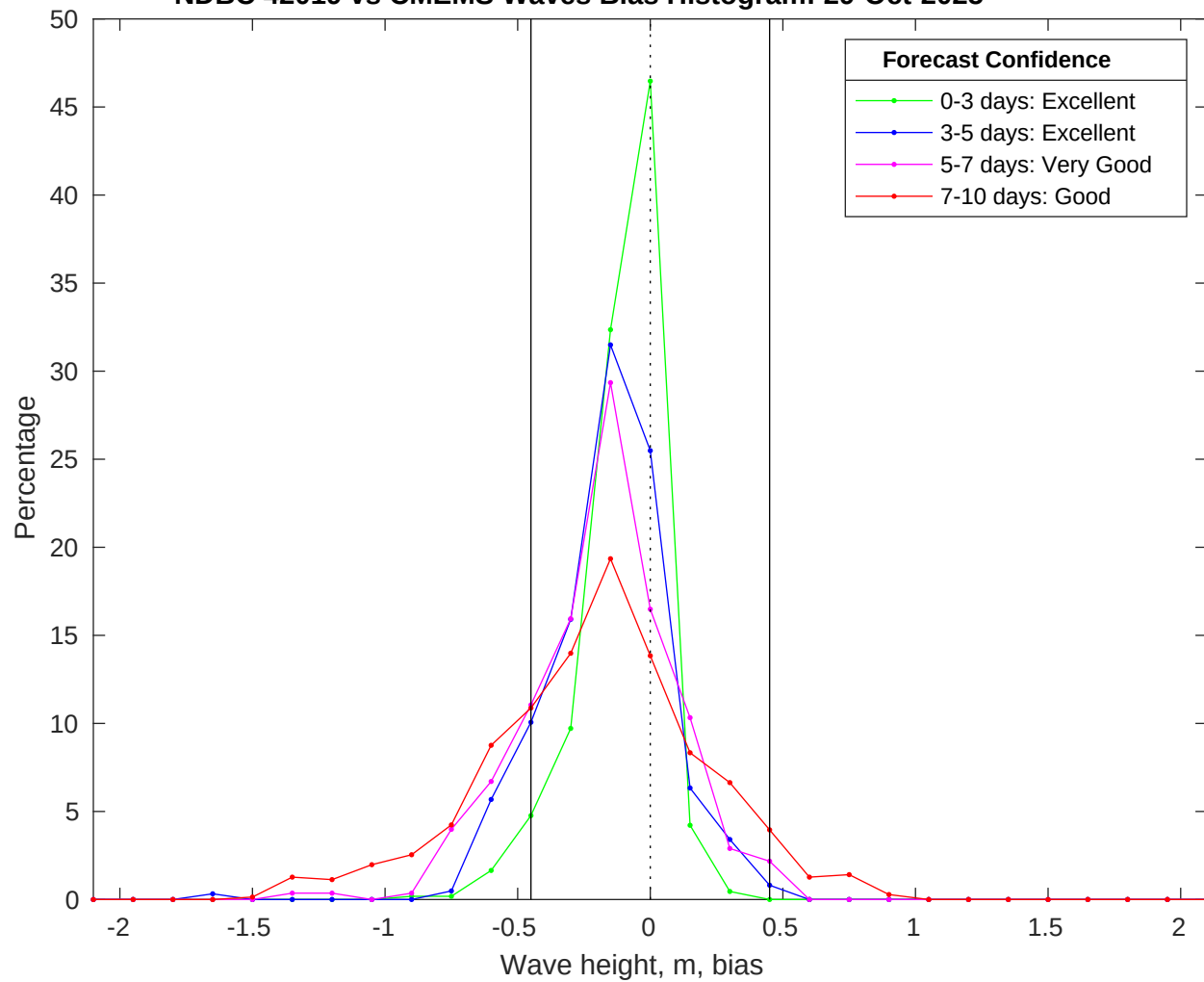
NDBC 42019 vs CMEMS Waves Bias Histogram: 29-Oct-2025
