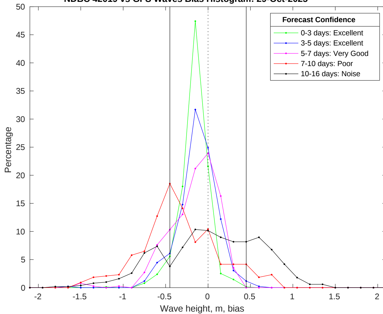
NDBC 42019 vs GFS Waves Bias Histogram: 29-Oct-2025
